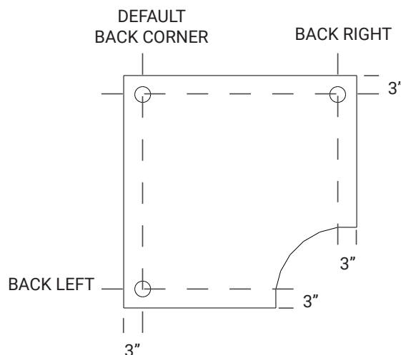
Corner Applications
