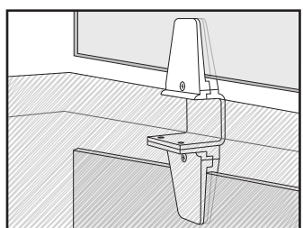
Bracket detail
