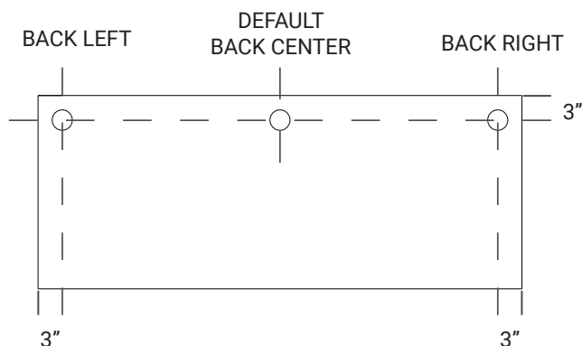
Rectangular Applications
