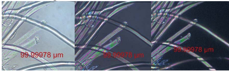
Figure 1: Synthetic fibers damaged with a bullet and nail gun viewed under plane polarized light (left), 65° crossed polarizers (middle) and 90° crossed polarizers (right). Magnification x400.
