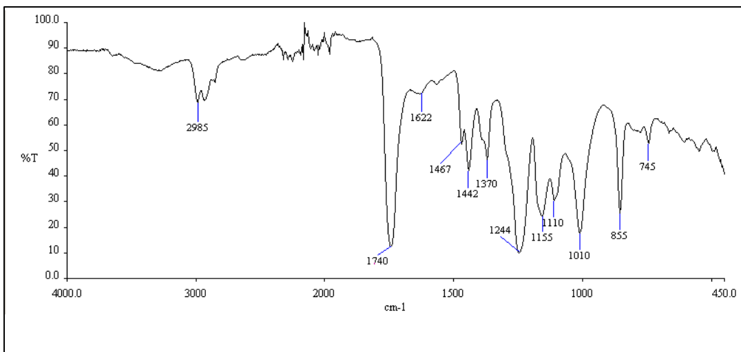
Figure 1. FTIR spectra of cyanoacrylate
