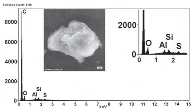
Figure 22. NIST bituminous coal, SEM.
