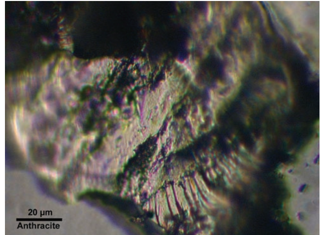
Figure 2. Anthracite coal, reflected light.
